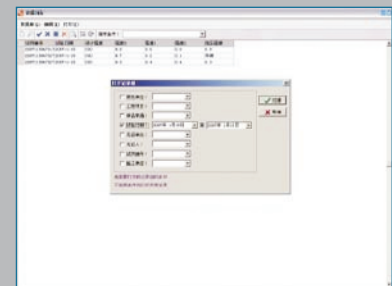
Database management
