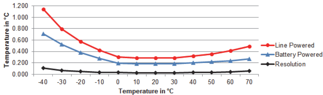
Plot A: Accuracy Range of ZW-001 Integrated Temperature Sensor
