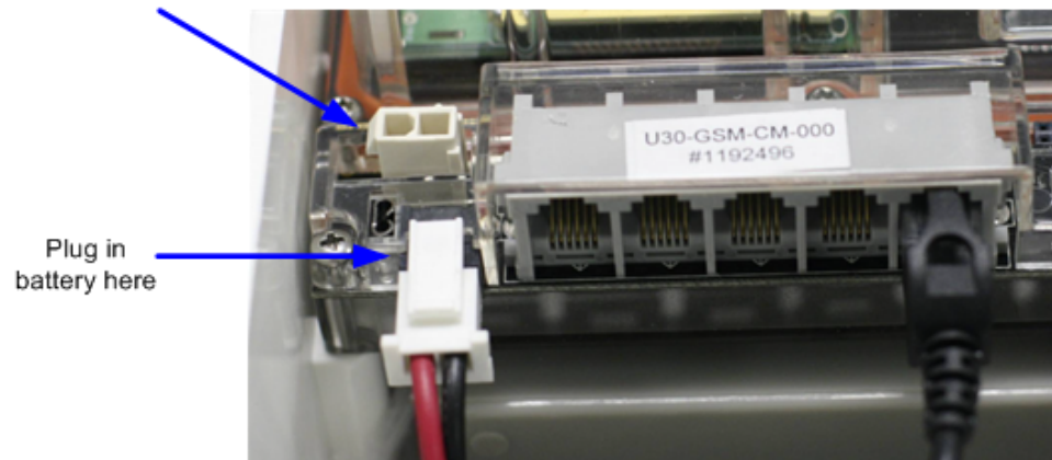
Figure 31: Connecting the Battery
