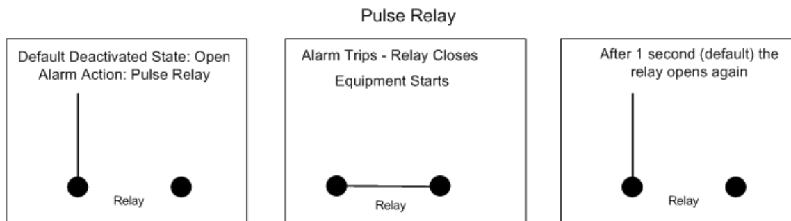
Figure 20: Pulse Relay
