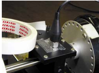
Secure the sensor with double-sided adhesive tape.
